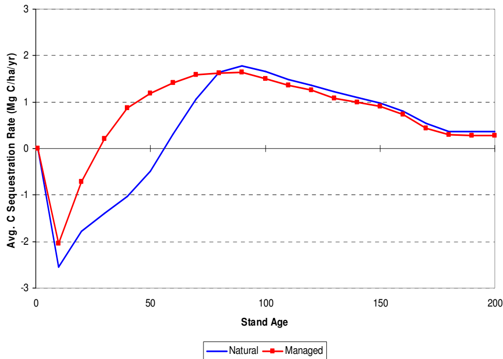
Figure 14: An Example of Average C Sequestration Rates for a Natural Spruce Leading Site Index 17 Stand (Forecast AU 3) and an Associated Managed Stand (Forecast AU 34)
